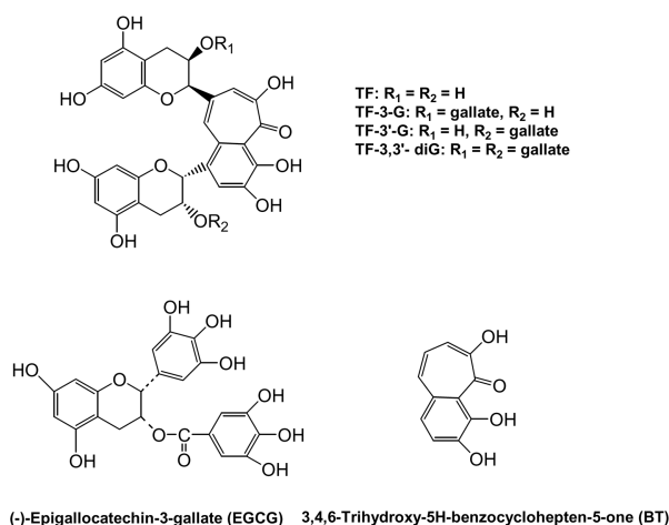
Figure 1. Chemical structures of green tea EGCG, black tea TFs, and 3,4,6-trihydroxy-5H-benzocyclohepten-5-one (BT).
